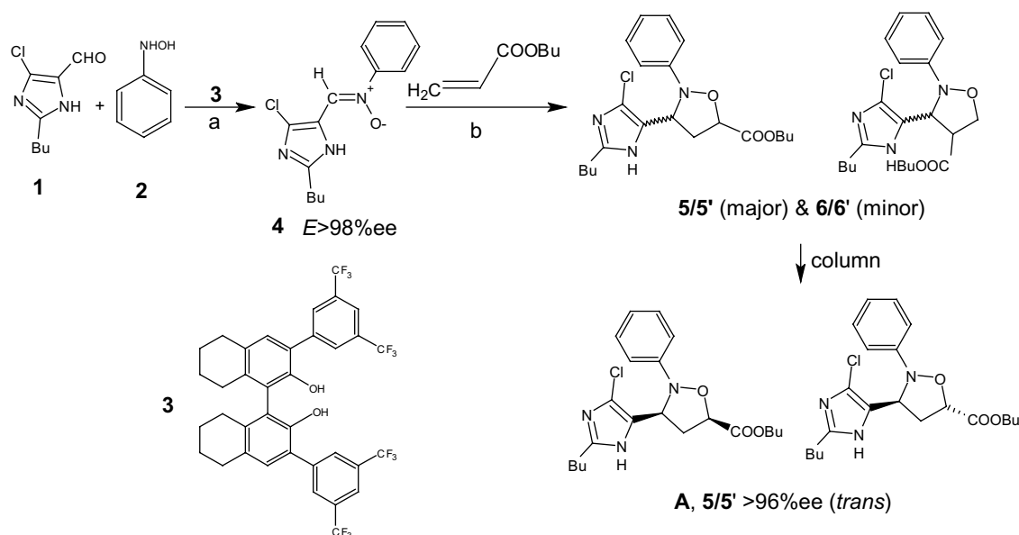
Scheme 1. Reagents and conditions: (a) \text{MgCl}_2 , methylene dichloride; (b) toluene, reflux, 38 h.
