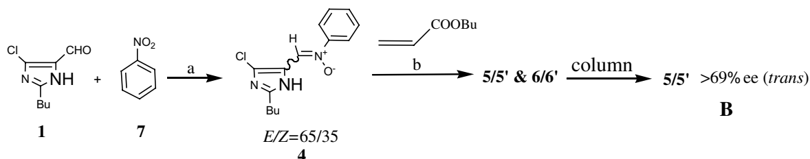
Scheme 2. Reagents and conditions: (a) \text{H}_2\text{O} :ethanol:DMF (7:2:1), zinc dust, -5^\circ\text{C} , pH 7.2–7.4; (b) toluene, reflux, 38 h.
